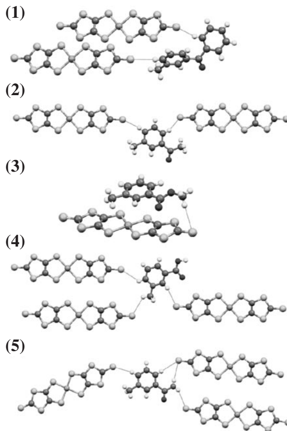
Figure 4. C–H...S and N–H...S hydrogen bonds between a cation and surrounding anions in 1–5, shown by dashed lines.
