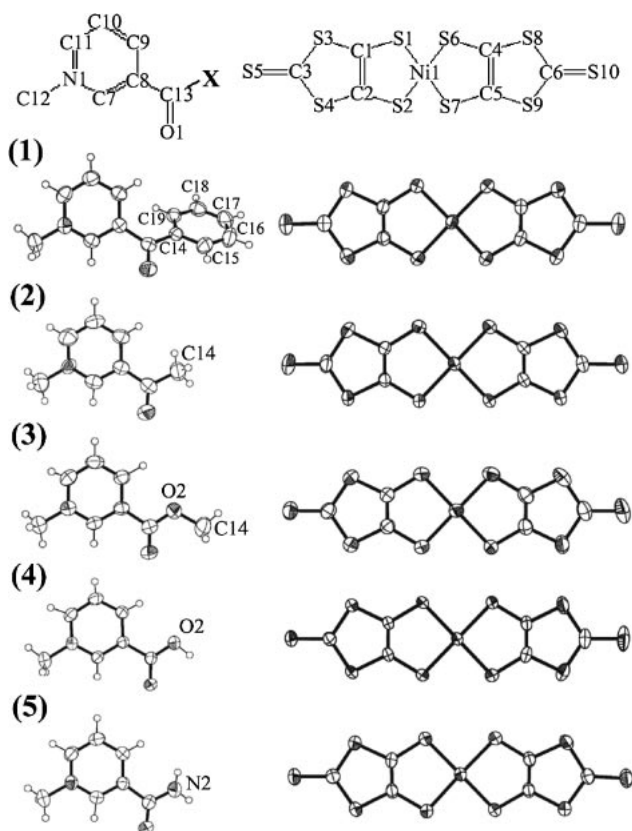
Figure 1. ORTEP III views of 1–5 , showing 50% probability ellipsoids with atom numbering scheme.
