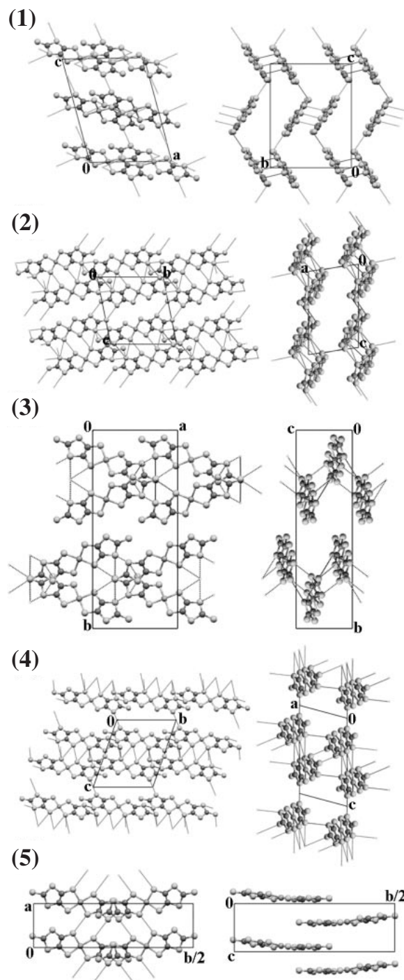
Figure 2. Crystal packing of [\text{Ni}(\text{dmit})_2] anions in 1–5 viewed along two different directions; Dashed lines indicate the short S...S contacts.
