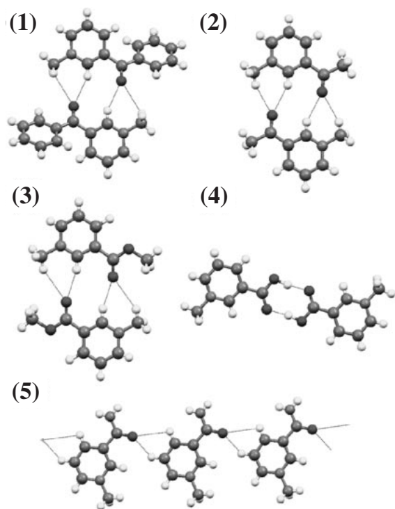
Figure 3. C–H...O and O–H...O hydrogen bonds between the cations in 1–5, shown by dashed lines.
